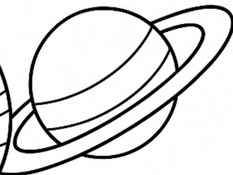
Saturn
